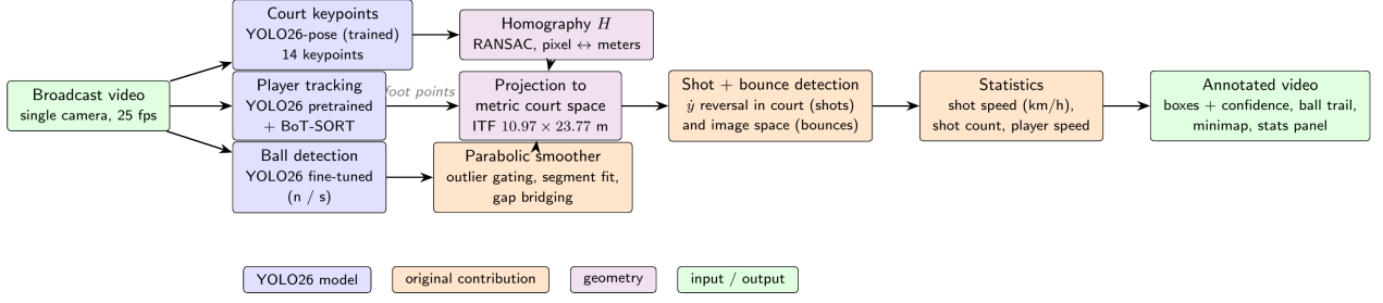
Figure 1: TennisVision pipeline. The input video is processed by three YOLO26 models: a pose model for the 14 court keypoints (from which the image-to-court homography is estimated), the pretrained detector with BoT-SORT association for the two players, and a fine-tuned detector for the ball. Ball detections are refined by a piecewise parabolic smoother, all positions are projected to metric court coordinates, shots are detected as motion reversals along the court length, and statistics are rendered on the annotated output video with a top-down minimap.
